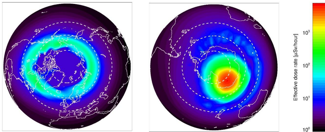
Figure 13: Calculated effective dose rate at 250 \text{ g/cm}^2 (ca. 10.5 km, 34 000 ft) over the northern hemisphere (left) and over the southern hemisphere (right) during the maximum phase of GLE69 based on GLE parameters determined from the data of the worldwide network of NM stations.
