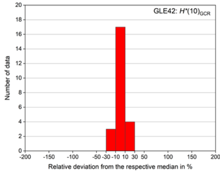
GLE42: GCR, H^*(10) , 11% ( 1\sigma )
