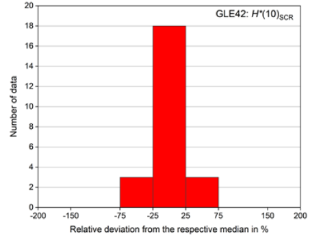
GLE42: SCR, H^*(10) , 29% ( 1\sigma )
