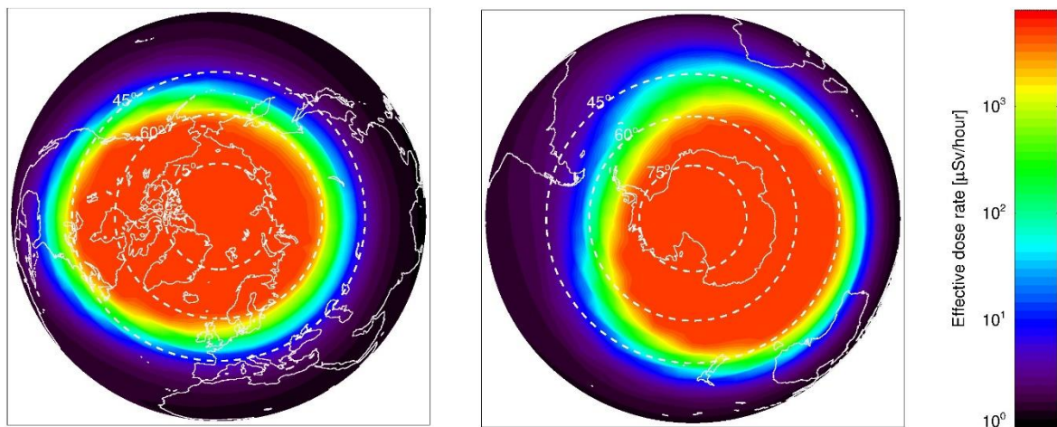
Figure 14: Calculated effective dose rate at 250 \text{ g/cm}^2 over the North hemisphere (left) and over the South hemisphere (right) during the maximum phase of GLE69 with the assumption of isotropic solar cosmic ray flux near Earth.
