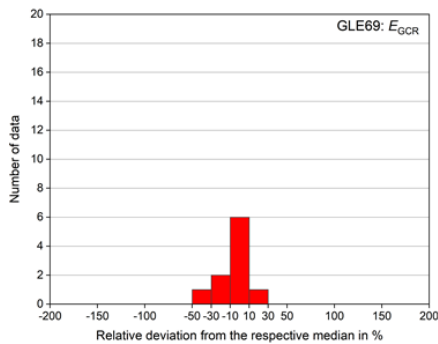
GLE69: GCR, E , 14% ( 1\sigma )
