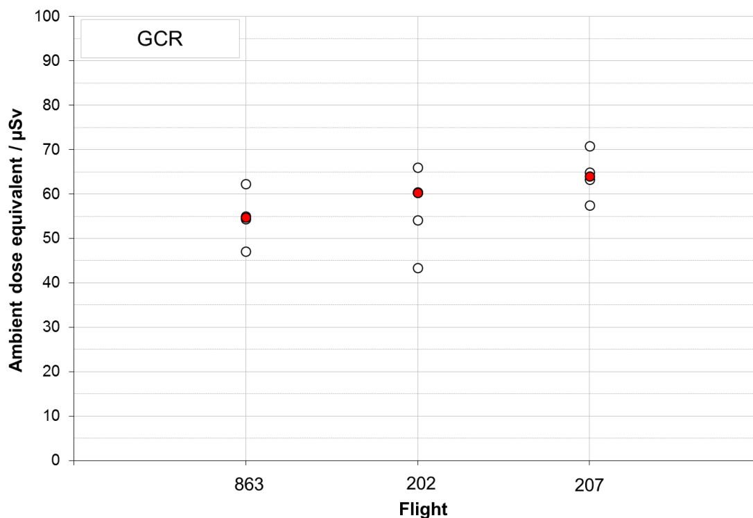
Figure 35: Comparison of route ambient dose equivalent for galactic cosmic radiation (GCR) calculated with 1-minute resolution for selected flights (white) presented with the median (red).
