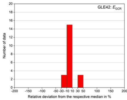
GLE42: GCR, E , 17% ( 1\sigma )
