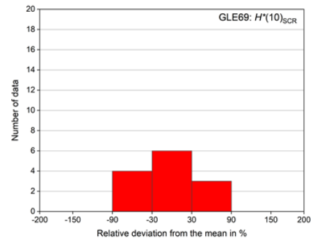
GLE69: SCR, H^*(10) , 50% ( 1\sigma )
