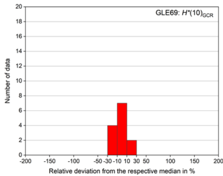
GLE69: GCR, H^*(10) , 11% ( 1\sigma )
