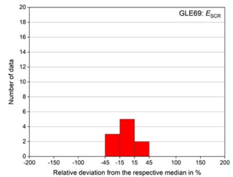
GLE69: SCR, E , 25% ( 1\sigma )
