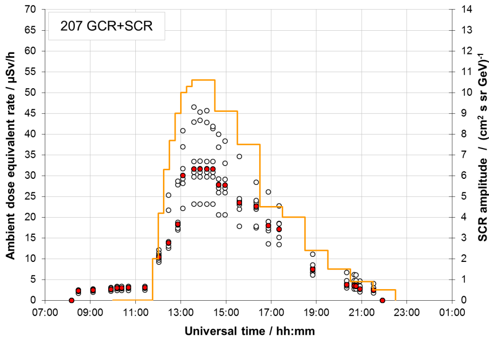
Figure 32: Comparison of ambient dose equivalent rate for the sum of galactic cosmic radiation (GCR) and “simplified GLE42” event (SCR) calculated for selected flight profile (207: Sydney–Johannesburg) by different codes (white, left axis) presented with median (red, left axis). In addition, we show the time profile of GLE42 (orange, right axis) event for solar protons with energies of 1 GeV near Earth, outside the geomagnetosphere as defined in Table 2.
