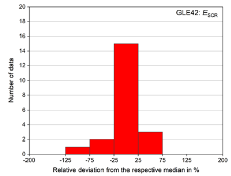
GLE42: SCR, E , 30% ( 1\sigma )
