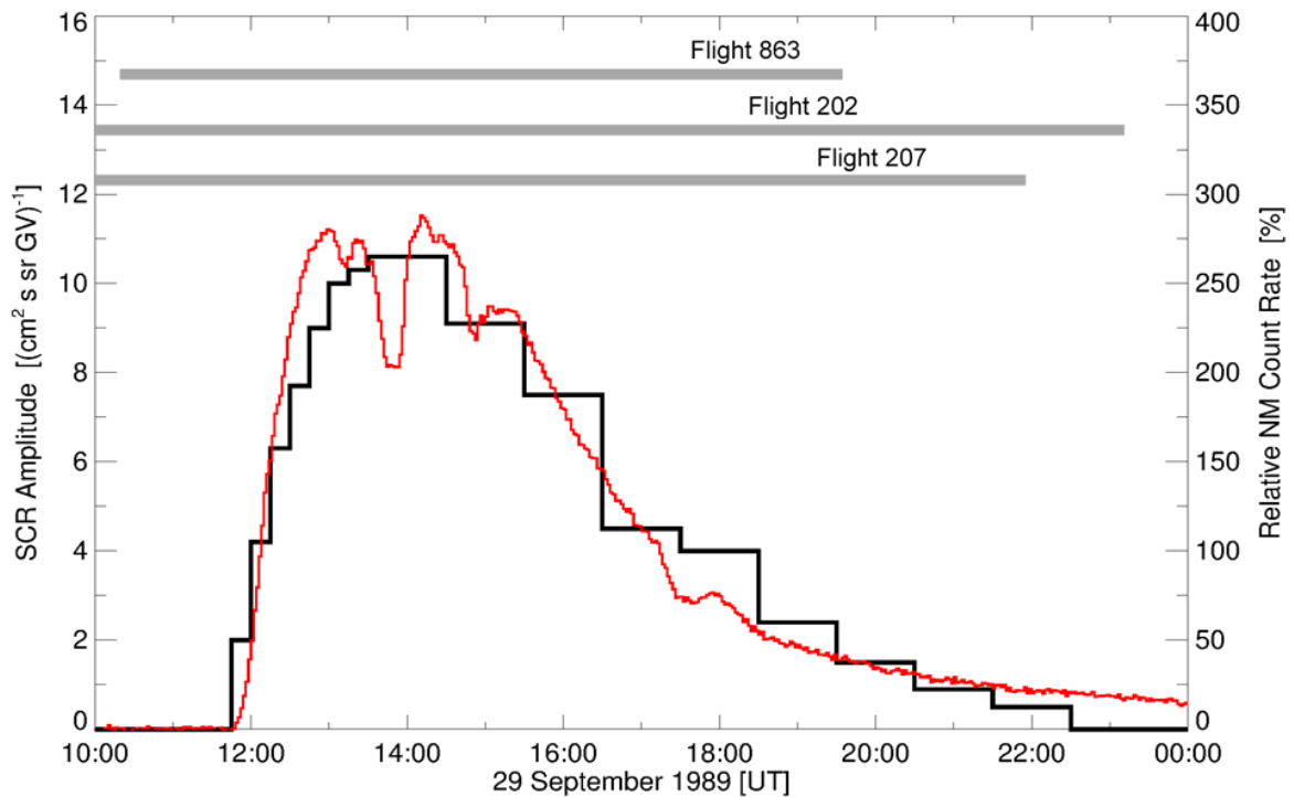
Figure 17: Amplitude of the solar cosmic ray flux at 1 GV as defined for the study of the simplified GLE42 on 29 September 1989, 10:00-24:00 UT (black line, see chapter 5.1.1). The horizontal grey bars indicate the adjusted flight times of the three investigated flights (for details see Appendix 2). For illustration the five-minute pressure corrected relative count rate of the neutron monitor at McMurdo, Antarctica, is also shown (red line, data source: NMDB).
