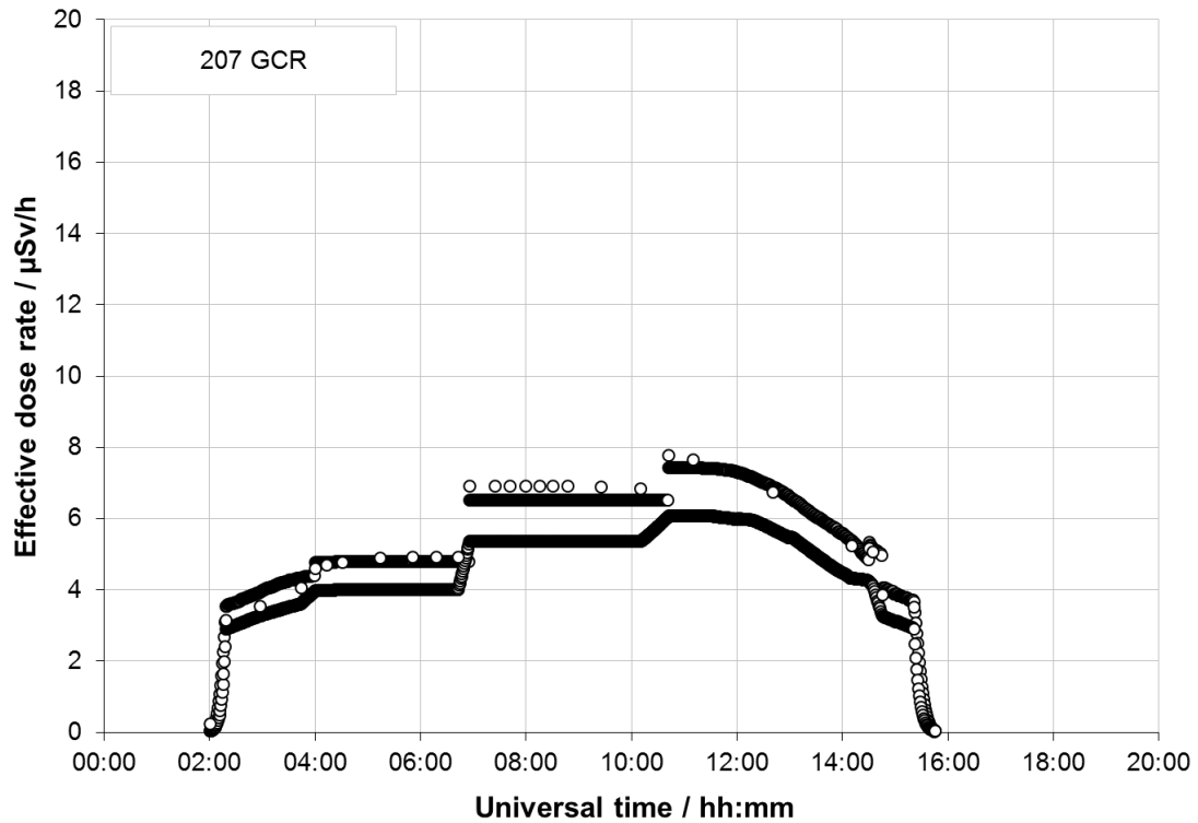
Figure 49: Comparison of effective dose rate for galactic cosmic radiation (GCR) calculated for selected flight profile (207: Sydney–Johannesburg) by three codes.
