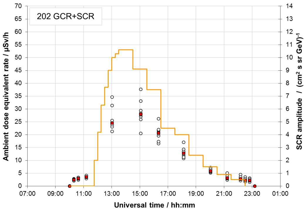
Figure 28: Comparison of ambient dose equivalent rate for the sum of galactic cosmic radiation (GCR) and "simplified GLE42" event (SCR) calculated for selected flight profile (202: Chicago–Beijing) by different codes (white, left axis) presented with median (red, left axis). In addition, we show the time profile of GLE42 event (orange, right axis) for solar protons with energies of 1 GeV near Earth, outside the geomagnetosphere as defined in Table 2.
